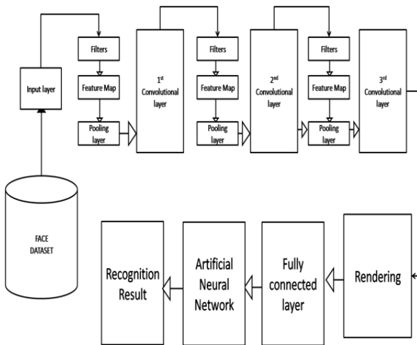
Figure 11: An Improved CNN Modeling Diagram
