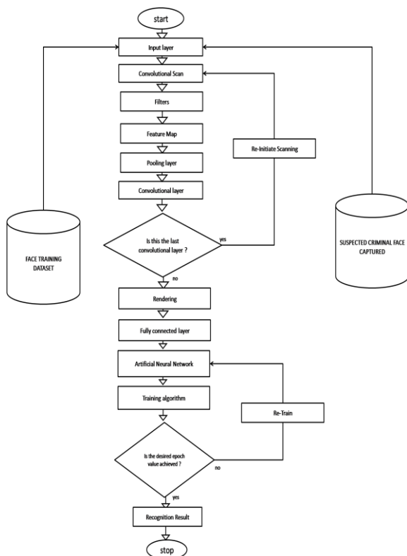
Figure 12: System Flowchart
