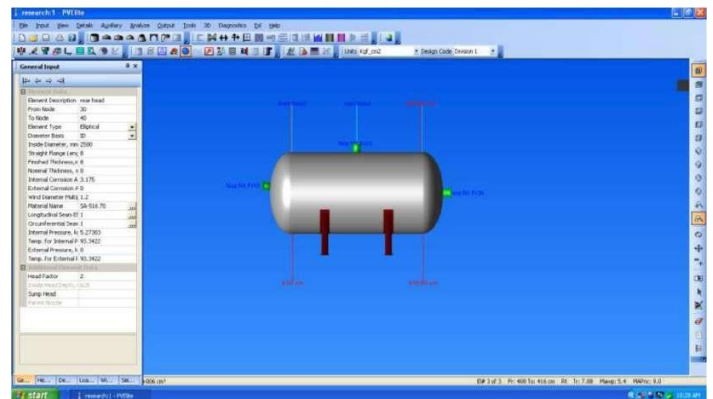
Figure 3 Mechanical Design of pressure vessel by PV ELITE
