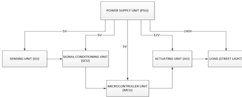
Figure1: Block Diagram of the Proposed Intelligent Street Light Controller
