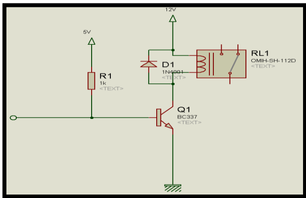
Figure 4: The Actuator Circuit
