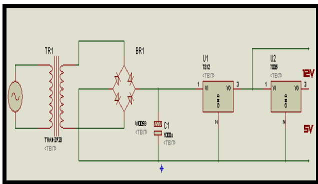
Figure 2: The Sub-circuit diagram of the Power Unit
