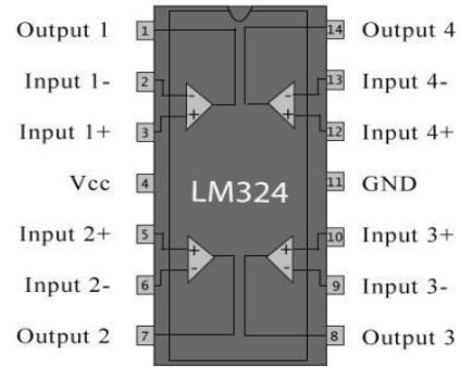
Figure 3: Pin Configuration of LM324
